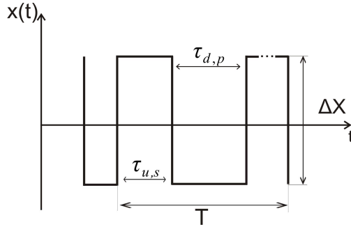
Fig. 1. Two-level RTS noise.
